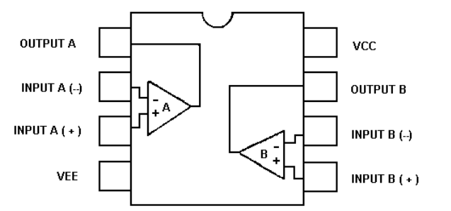
U501 344A3070P1 Operational Amplifier
