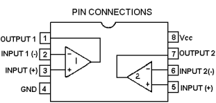
U302 & U601 19A116297P7 Dual Wide Band Op-Amp
