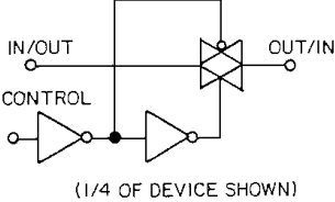
LOGIC DIAGRAM
